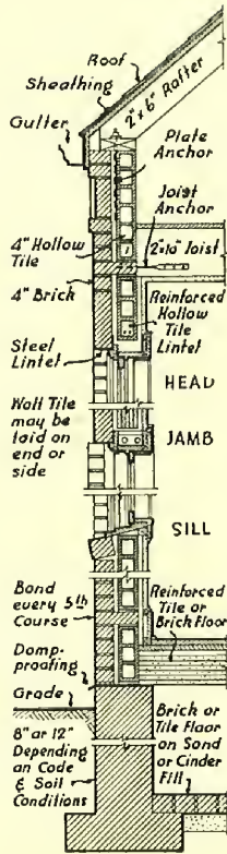
Wall Section
